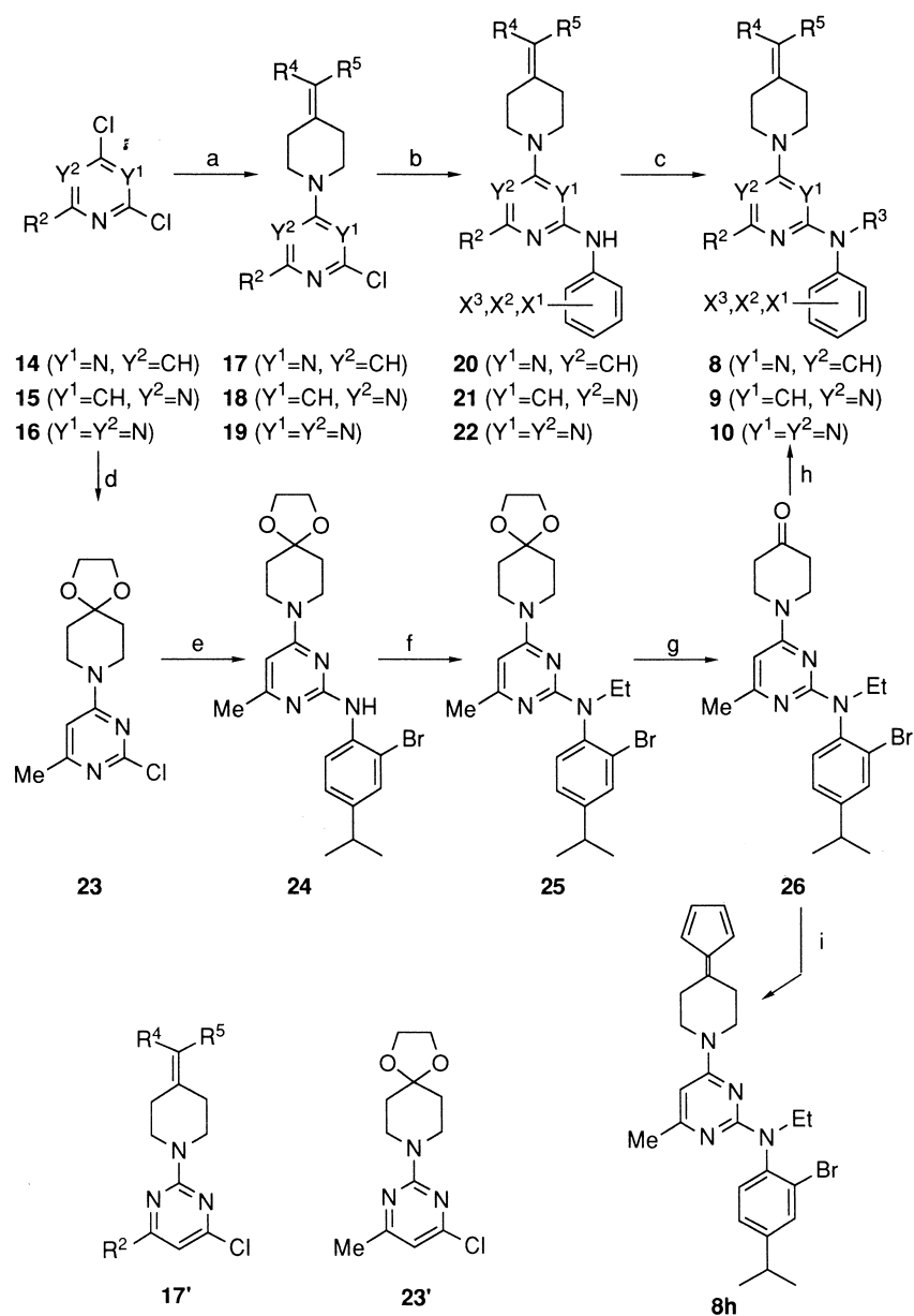
Scheme 1. Reagents and reaction conditions: (a) 4-( R^4, R^5C= )piperidine, isoPr_2NEt , EtOH; (b) X^3, X^2, X^1-Ar-NH_2 , isoPr_2NEt , (CH_2OH)_2 , reflux; (c) R^3-I or -Br , NaH, DMF; (d) 4-(1,3-dioxolan-2-yl)piperidine, isoPr_2NEt , EtOH; (e) 2-Br-4- isoPr-Ar-NH_2 , isoPr_2NEt , (CH_2OH)_2 , reflux; (f) Et-I, NaH, DMF; (g) 1 N Cl, THF; (h) R^4, R^5 = PPh_3 , THF; (i) cyclopentadiene, Et_3N . Method A: a, b, c; Method B: d, e, f, g; Method C: h; Method D: i.
