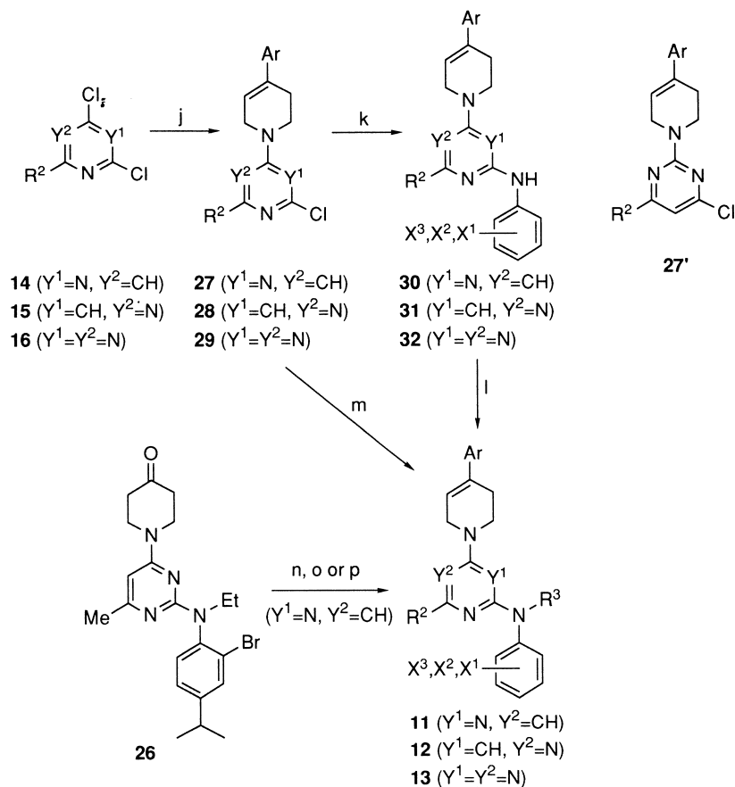
Scheme 2. Reagents and reaction conditions: (j) 4-Ar-1,2,3,6-tetrahydropyridine, iso Pr 2 NEt, EtOH; (k) X 3 , X 2 , X 1 -Ar-NH 2 , iso Pr 2 NEt, (CH 2 OH) 2 , reflux; (l) R 3 -I or -Br, NaH, DMF; (m) X 3 , X 2 , X 1 -Ar-NHR 3 , iso Pr 2 NEt, (CH 2 OH) 2 , reflux; (n) ArMg-Br or -I, THF, and then TFA-CH 2 Cl 2 ; (o) furan, LDA, THF and then MsCl, Et 3 N, DMAP, CH 2 Cl 2 ; (p) thiophene, LDA, THF and then HCO 2 H. Method E: j; Method F: k, l; Method G: m; Method H: n; Method I: o; Method J: p.
